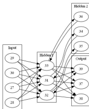
Neural Network
