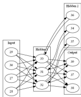
Neural Network
