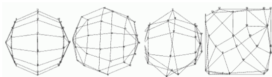
The two-dimensional representations of the 26 points on the sphere obtained by minimization of S , E , A , and by SOFM (left to right) with a 20 x 20 neurons map.
