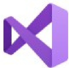
Visual Studio 2019
